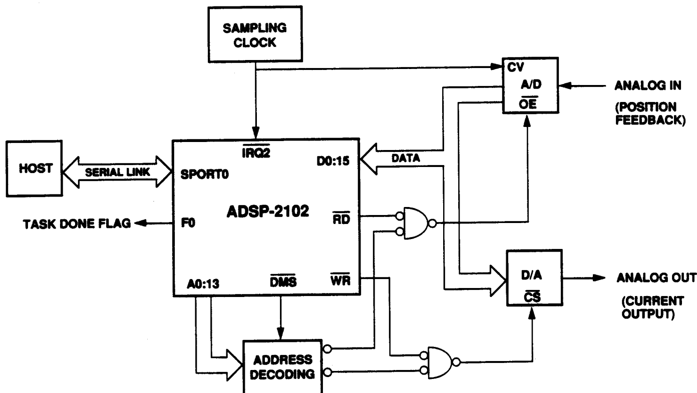
Figure 3. ADSP-2101 Based Actuator Controller
