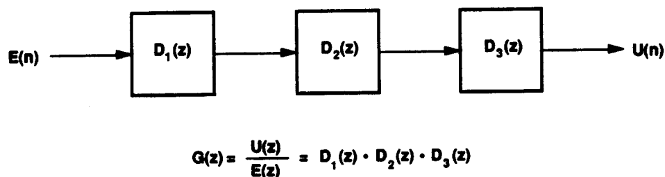
Figure 7. Cascaded Biquad Sections
